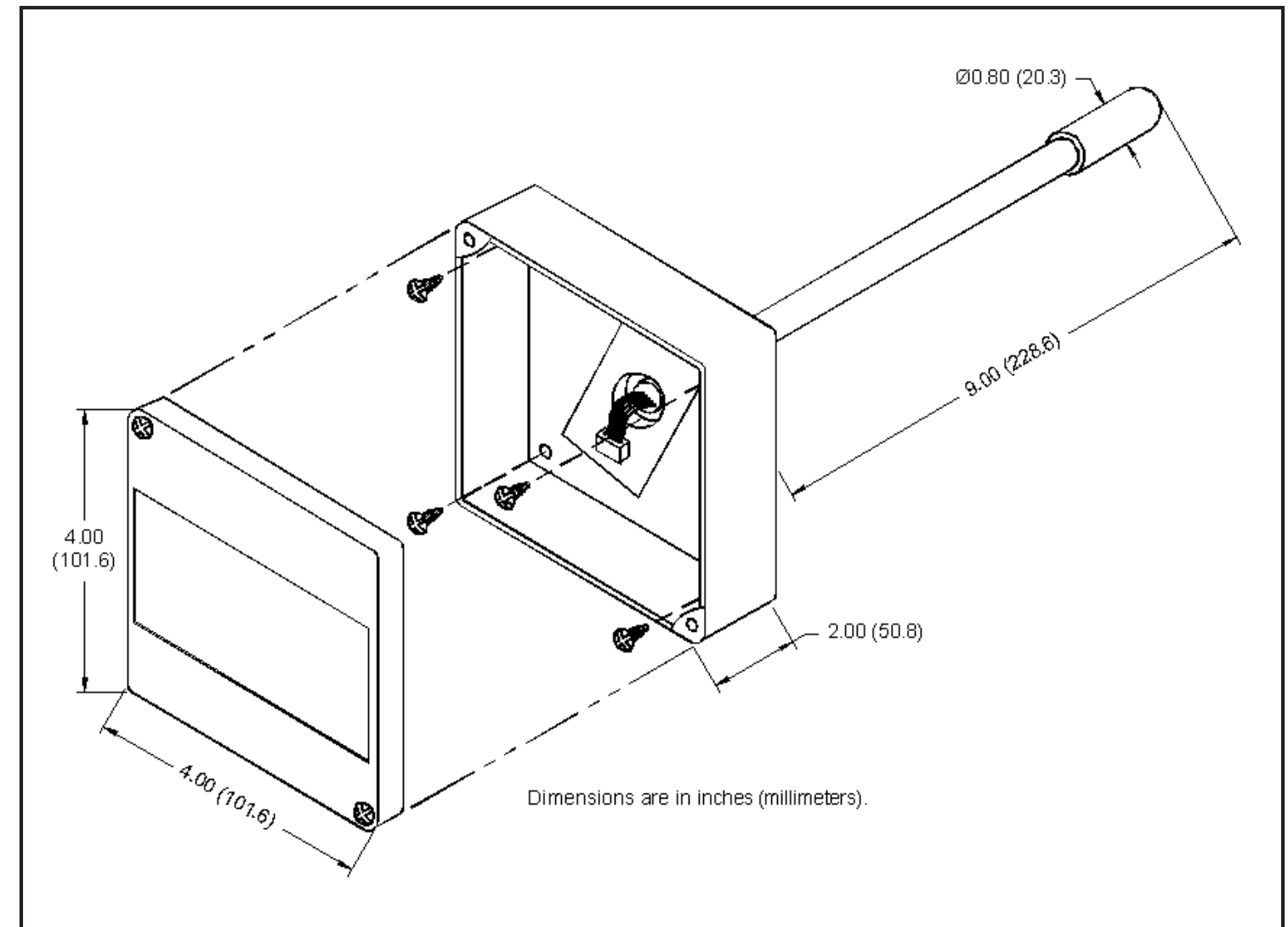
Figure 5: Duct Mount Dimensions
