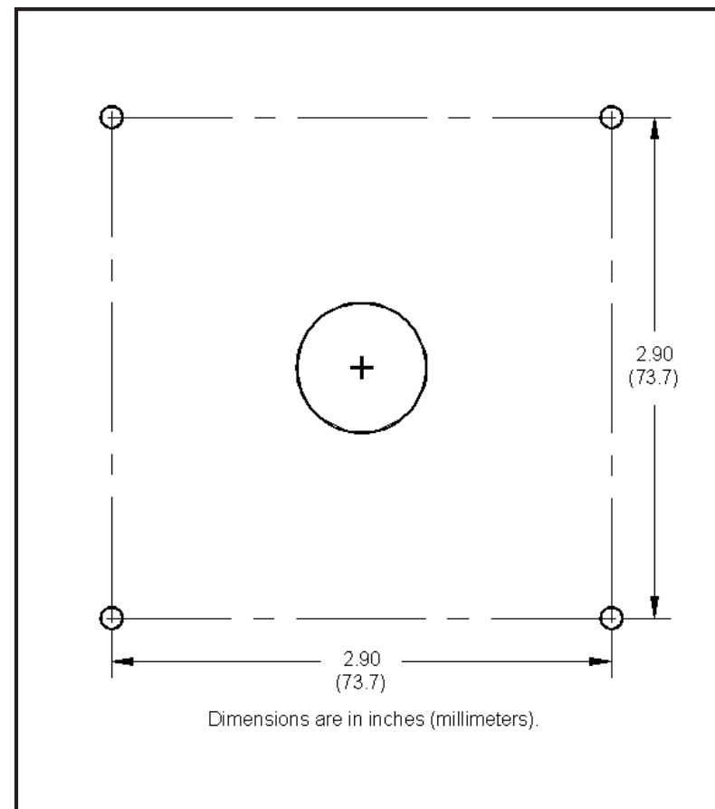
Figure 1: Duct Mounting Template - Full Size
