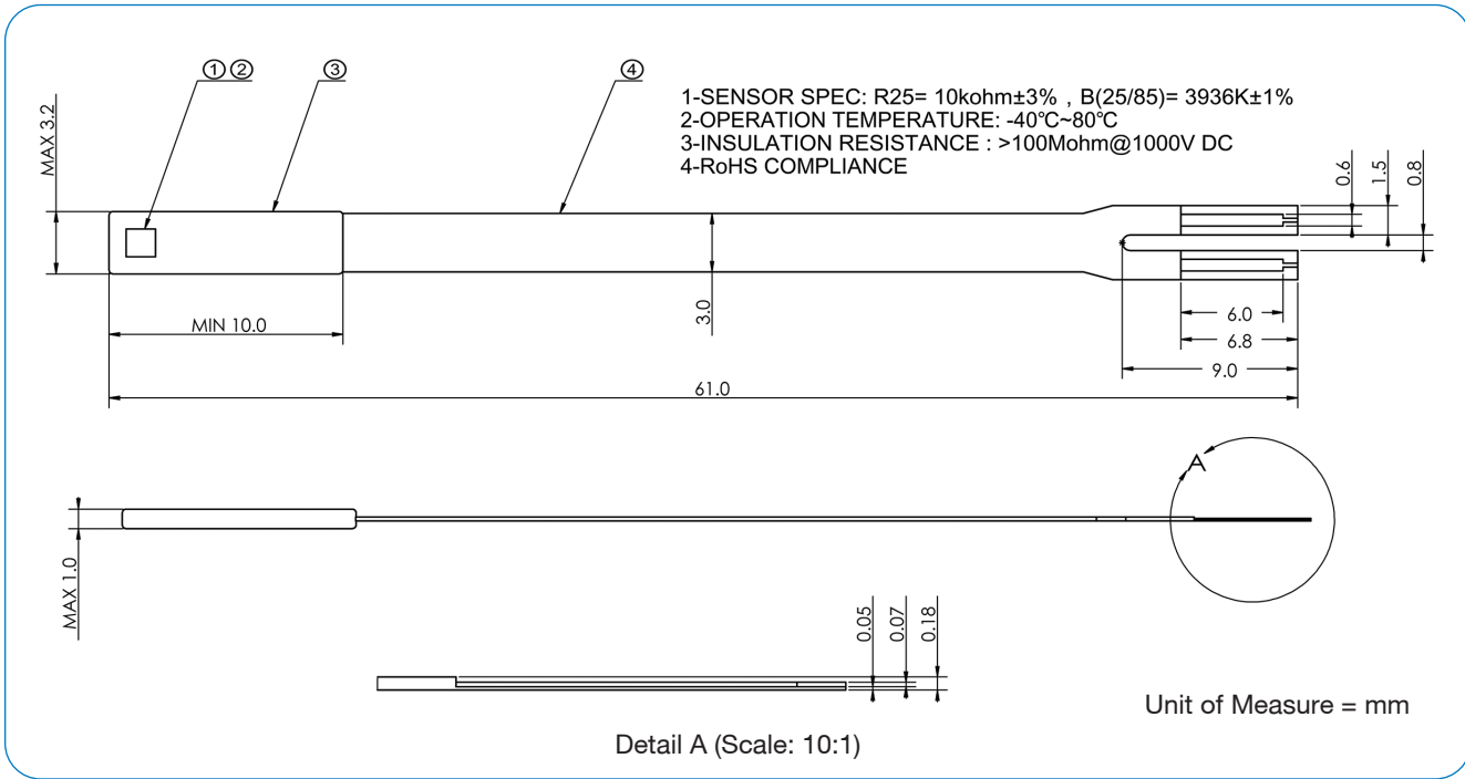
CTTS-203856-S02 Dimensions
