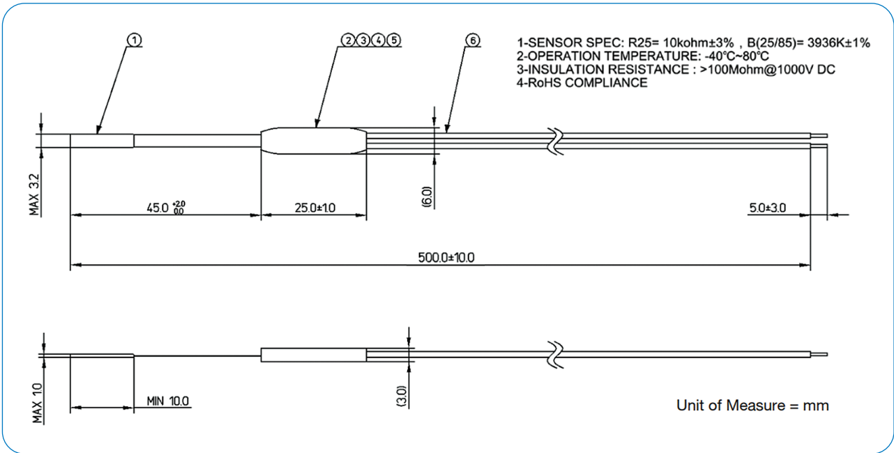
CTTS-203856-F04 Dimensions
