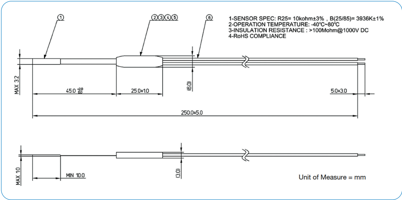
CTTS-203856-F03 Dimensions
